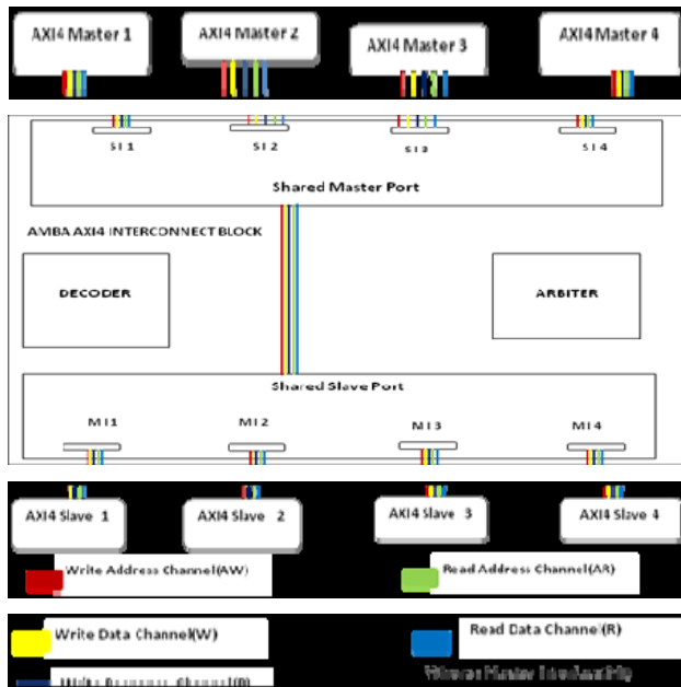
Fig3: Block Diagram of AMBA AXI4 Bus Interconnect.
