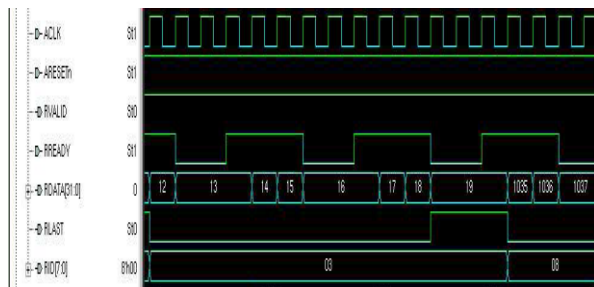
Figure 8: Simulation Result of Slave for Single Read Data Operation
