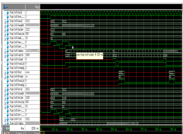
Figure 5: Simulation Result of Slave for Write Address & Write Data Operation.
