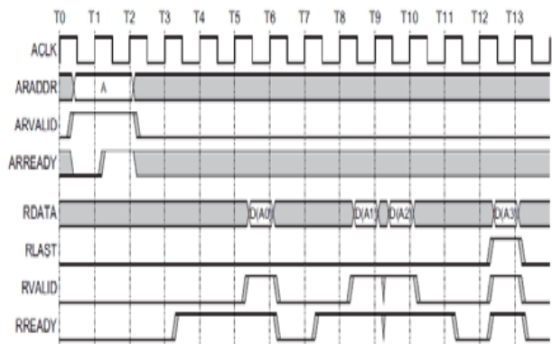
Figure 2: Read Address and Data Burst.
