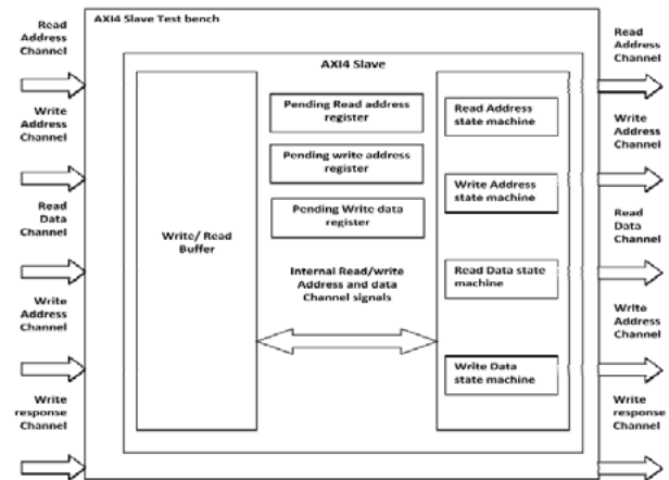
Fig 4: AMBA AXI4 Slave Read/Write Block Diagram
