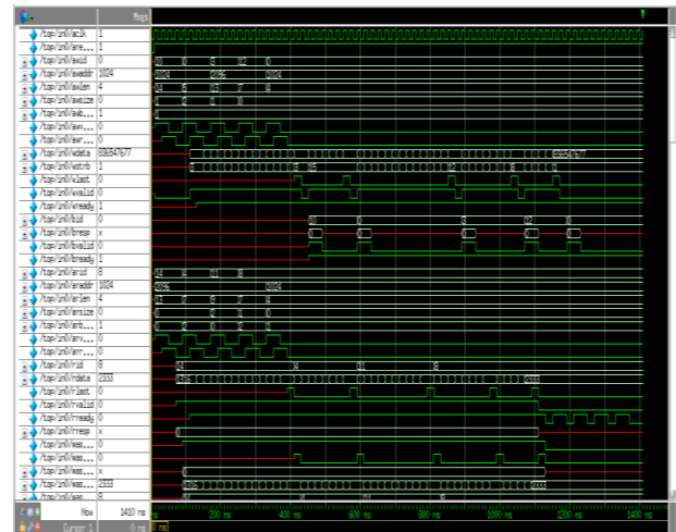
Figure 6: Simulation Result of Slave for Multiple Write Data Operation
